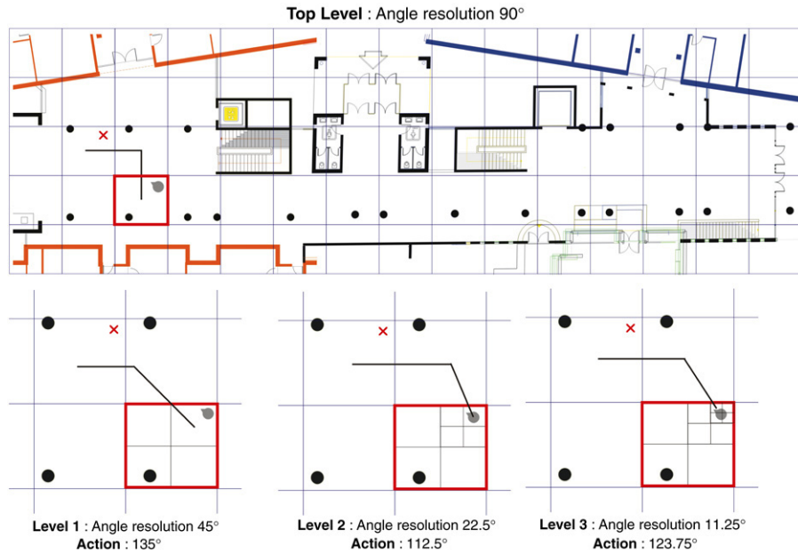
Fig. 5. Planning with the RN-HPOMDP.
